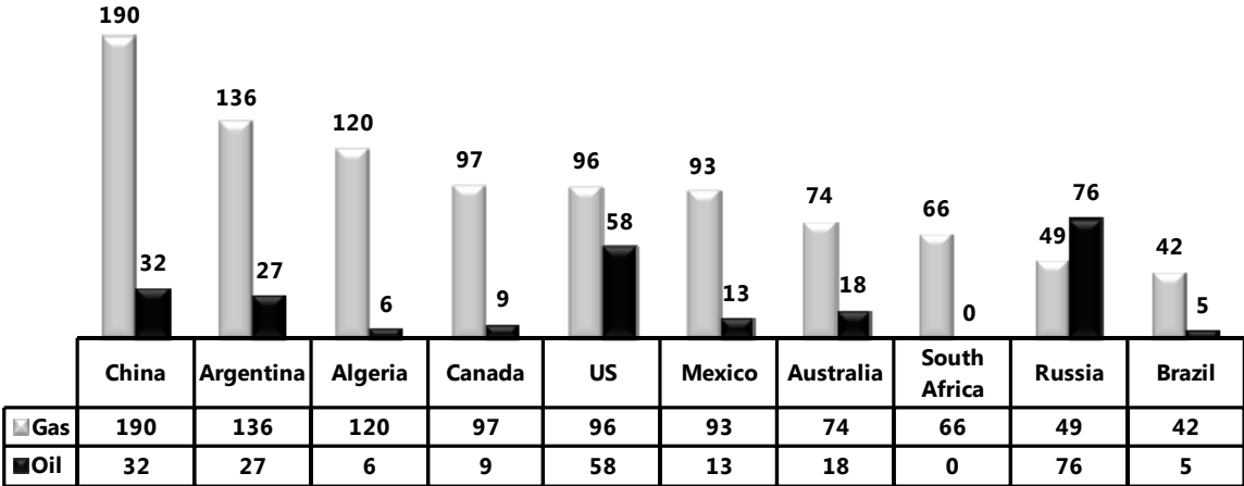
Figure 8 – World distribution of shale oil & gas in place (in Gboe). (EIA)
