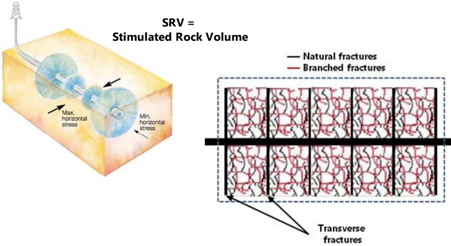
Figure 3 – Multi-fracturing of a horizontal well. SRV concept.
