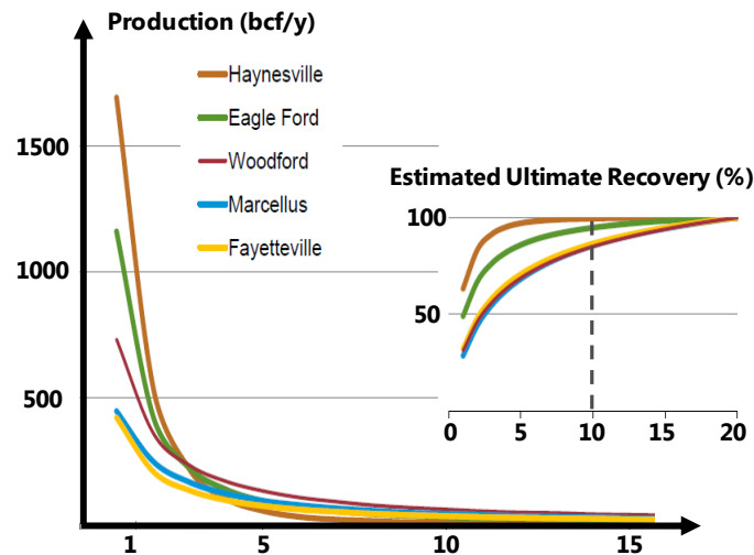
Figure 6 – Typical decline curves of US shale gas wells (according to IHS CERA)
